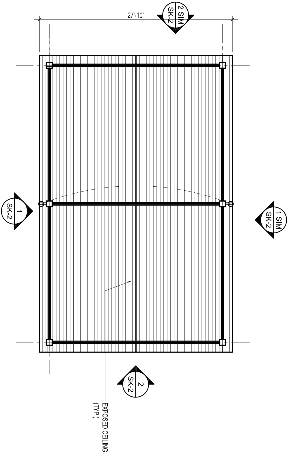
A ELECTRICAL OUTLET PLAN SCALE: 1/8" = 1'-0"
